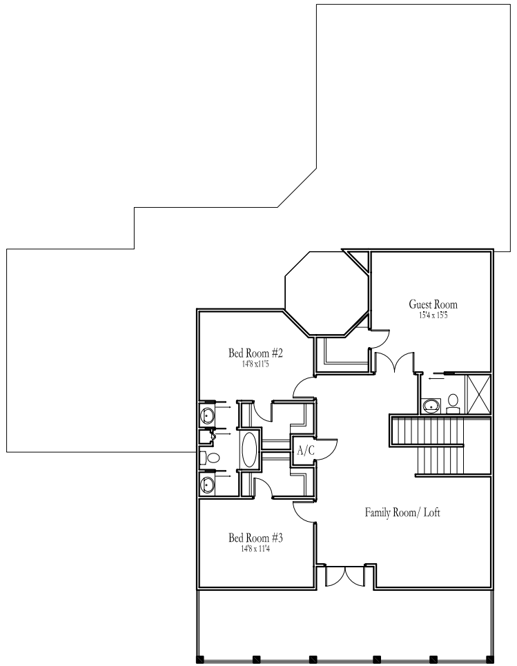
Second Floor Plan N.T.S
