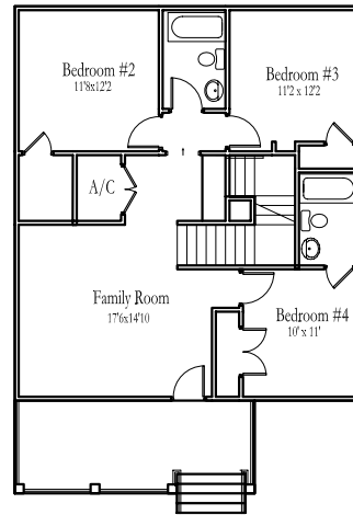
Second Floor Plan N.T.S
