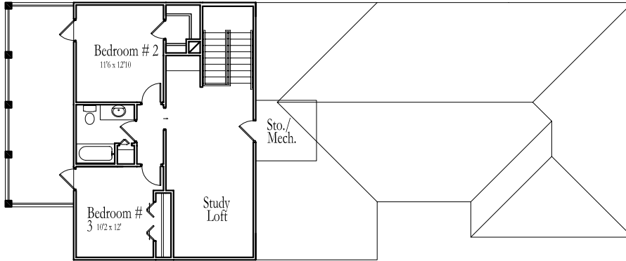
Second Floor Plan N.T.S
