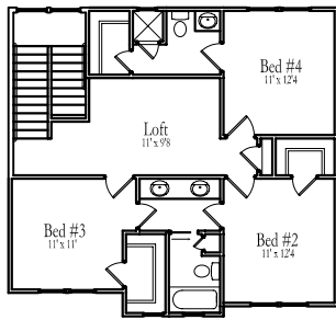
Second Floor Plan N.T.S.
