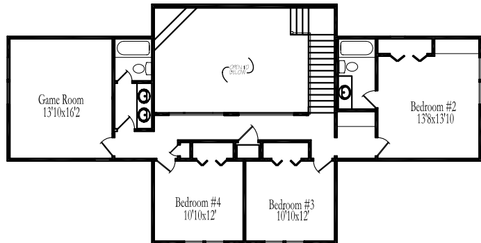
Second Floor Plan N.T.S
