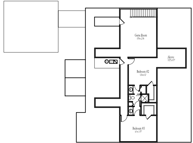
Second Floor Plan N.T.S
